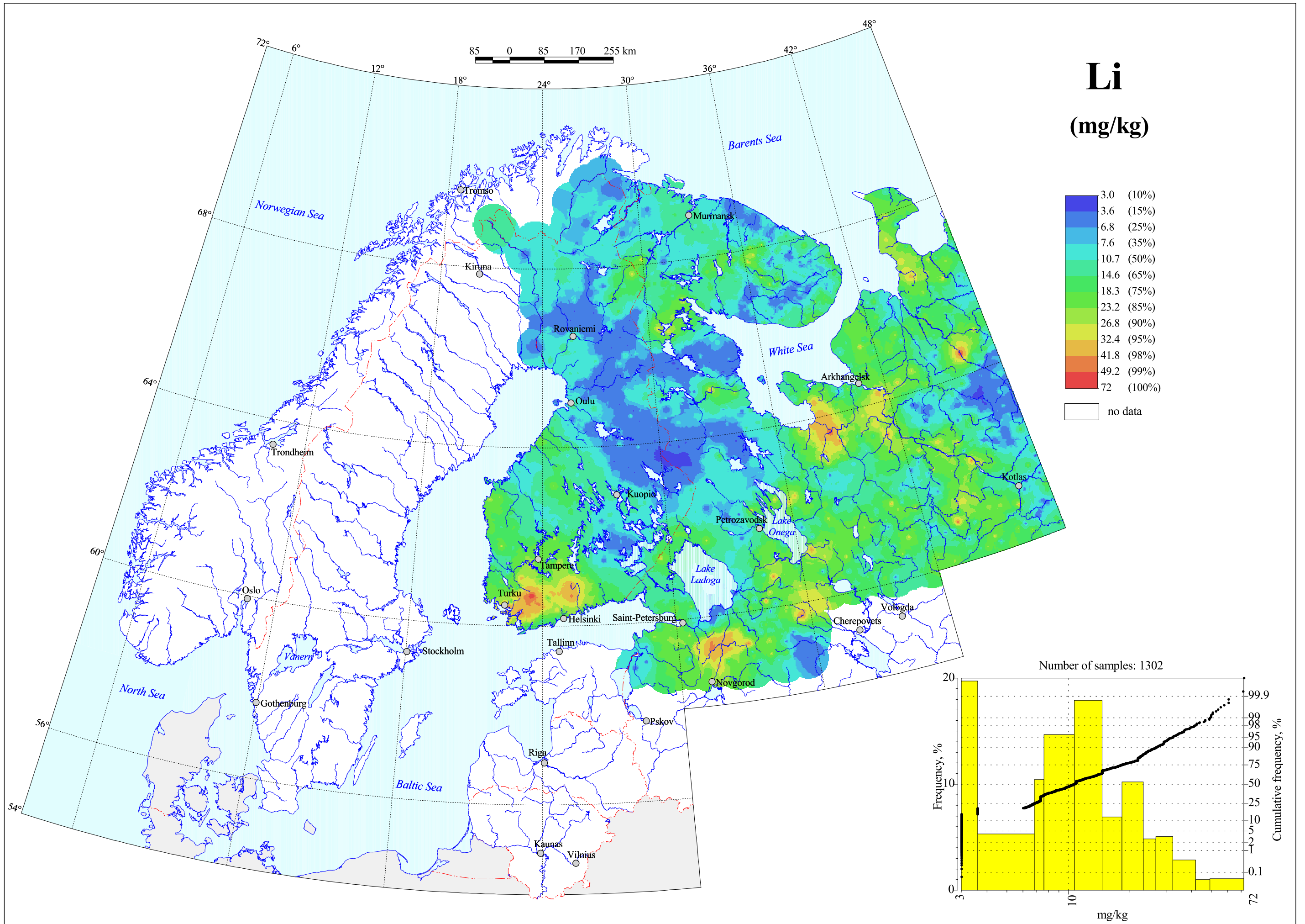
Lithium in C-horizon, Grain Size <2 mm, Total Content
